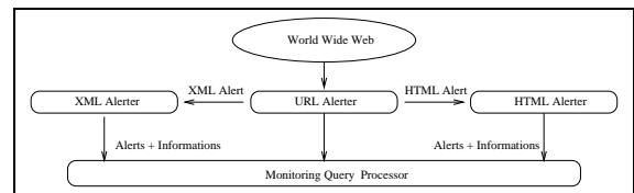
Figure 7: Overview of Alerters architecture
