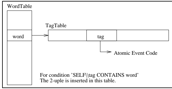
Figure 8: Registering ( Tag, Word ) conditions
