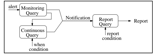
Figure 2: Main Components of the Subscription System
